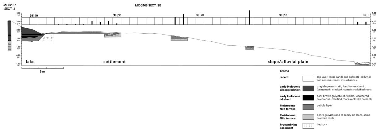
Fig. 6: MOG106, SE section. Trench 1 in relation to the absolute height of the stratigraphy at the neighbouring site MOG107 (left), the amount of lithic finds per square is indicated in the statistics given above (field recording: A. Dittrich, K. Geßner, M. Ehlert, H. M. Alkhidir Ahmed; drawing: A. Dittrich)
