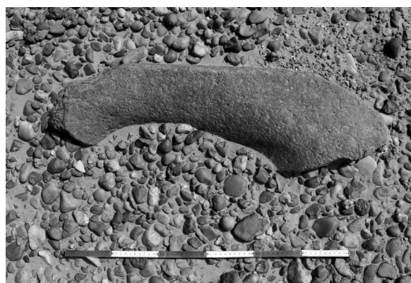
Fig. 21: MOG133. Half of a grinding base partly covered by serir (photo: A. Dittrich)
