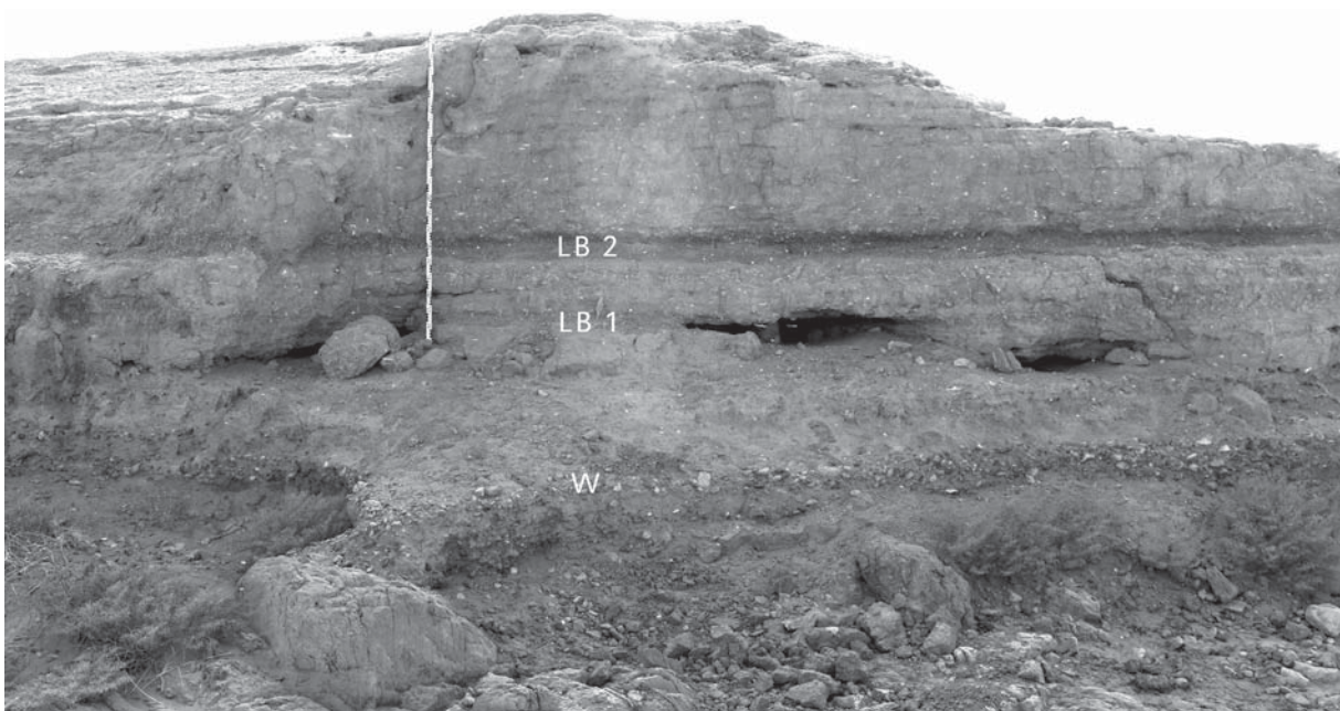
Fig. 16: Natural section at site MOG107 showing a sequence of wadi activity (W) and at least two early Holocene lakebeds (LB, length of scale: 2 m)
