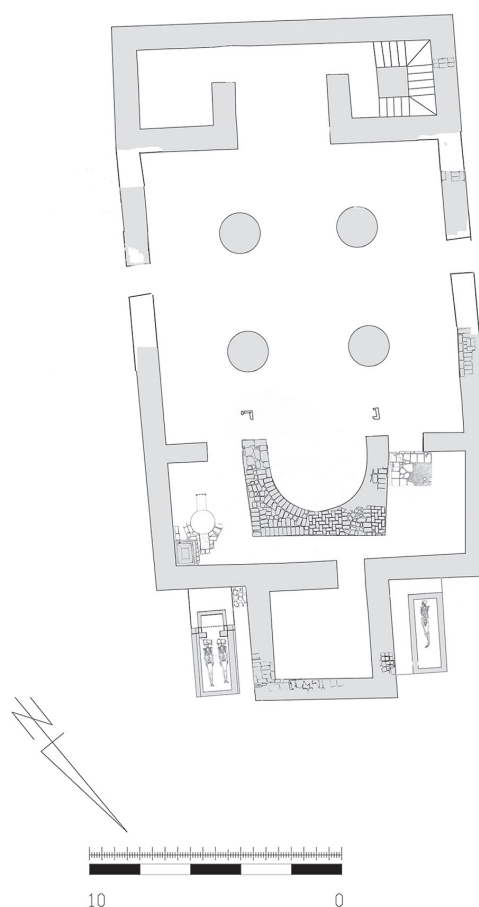
Fig. 9: Plan of the LCH2 (drawing: Bogdan Żurawski; measurements: Roman Łopaciuk).
